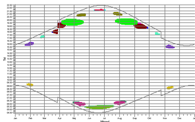
12: VESTAS V126-3.3 3300 126.0 !O! nav: 87,0 m (TOT:150,0 m) (221)
