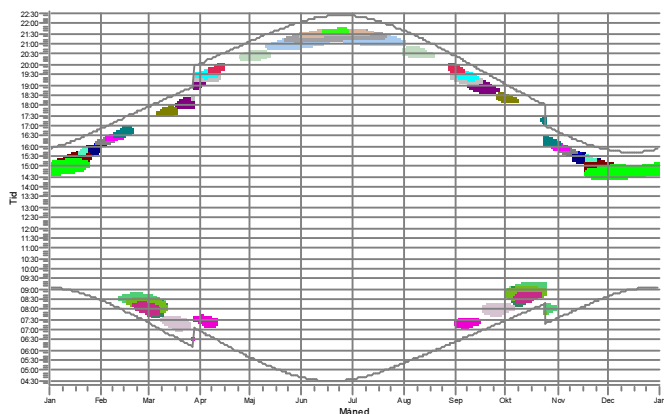
9: VESTAS V126-3.3 3300 126.0 !O! nav: 87,0 m (TOT:150,0 m) (218)
