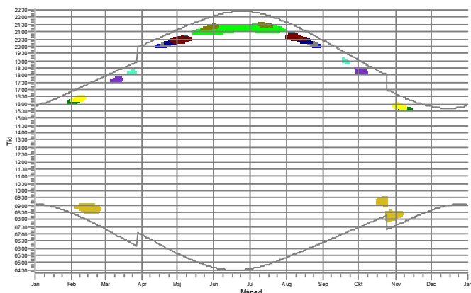
7: VESTAS V126-3.3 3300 126.0 !O! nav: 87,0 m (TOT:150,0 m) (216)
